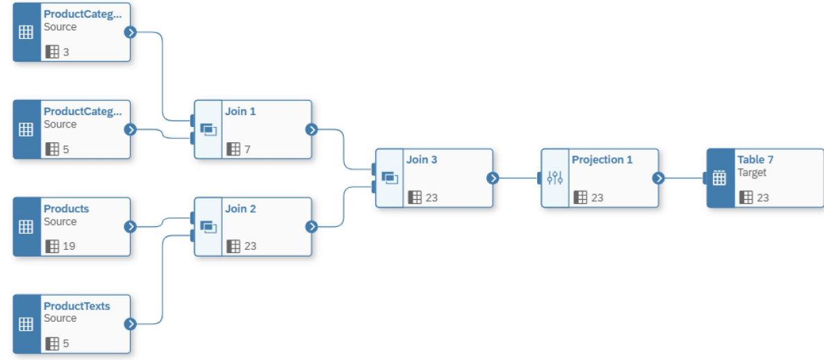
Data Flow Graphical Interface
