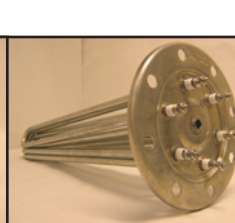
Element 12kW 230/400V 13Ω 30835,02
