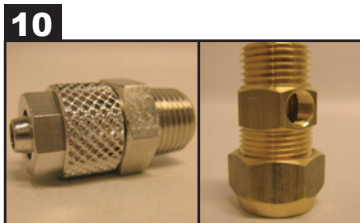
Koppling Rapid 1000 6/4-1/8 706,0902
