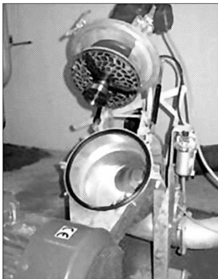
Figure: Perforated disc macerator and external shredder (Photo: Hugo Vögelsang Maschinenbau GmbH, KWS)
