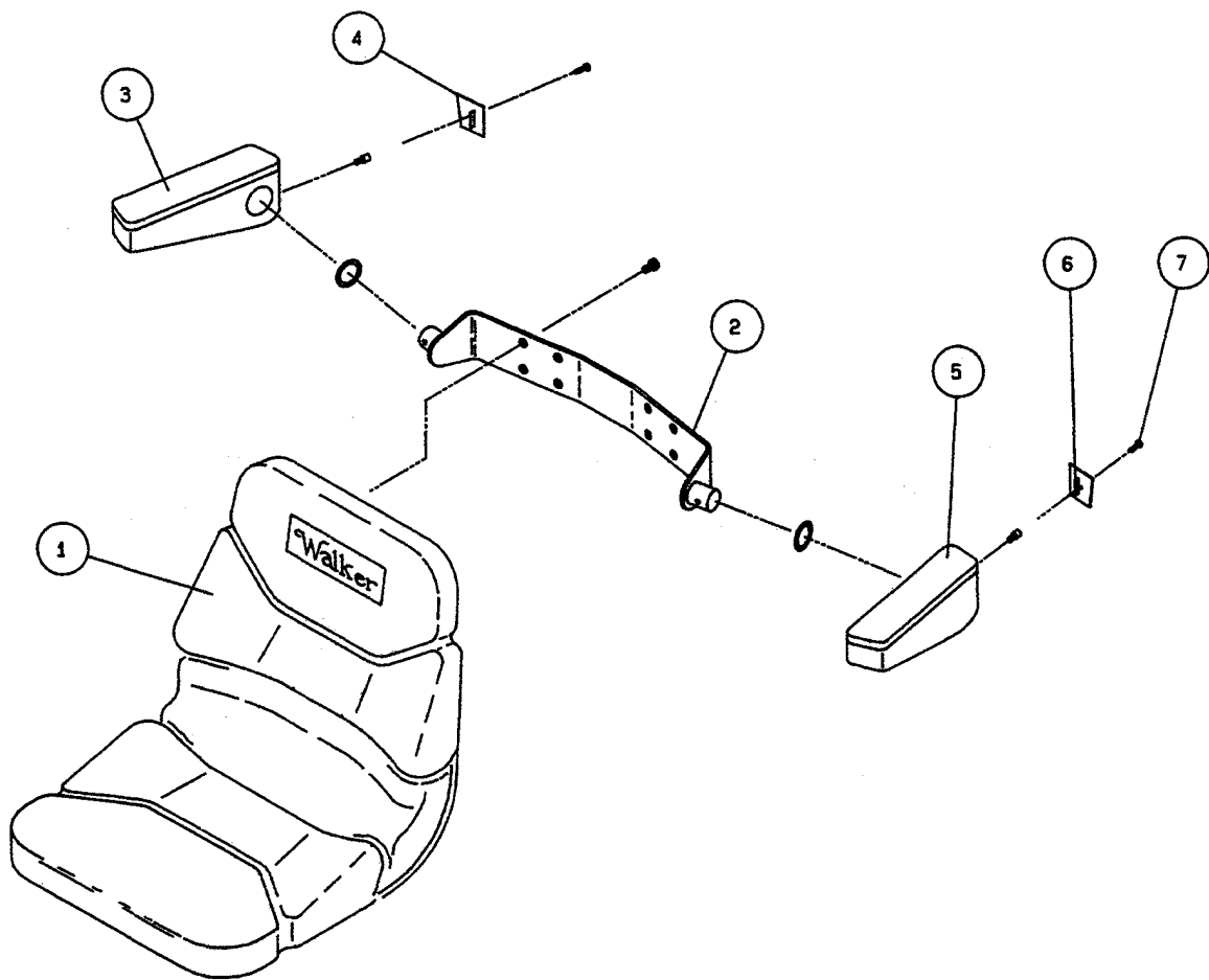
Figure K4 5885 Arm Rest Kit Assembly
