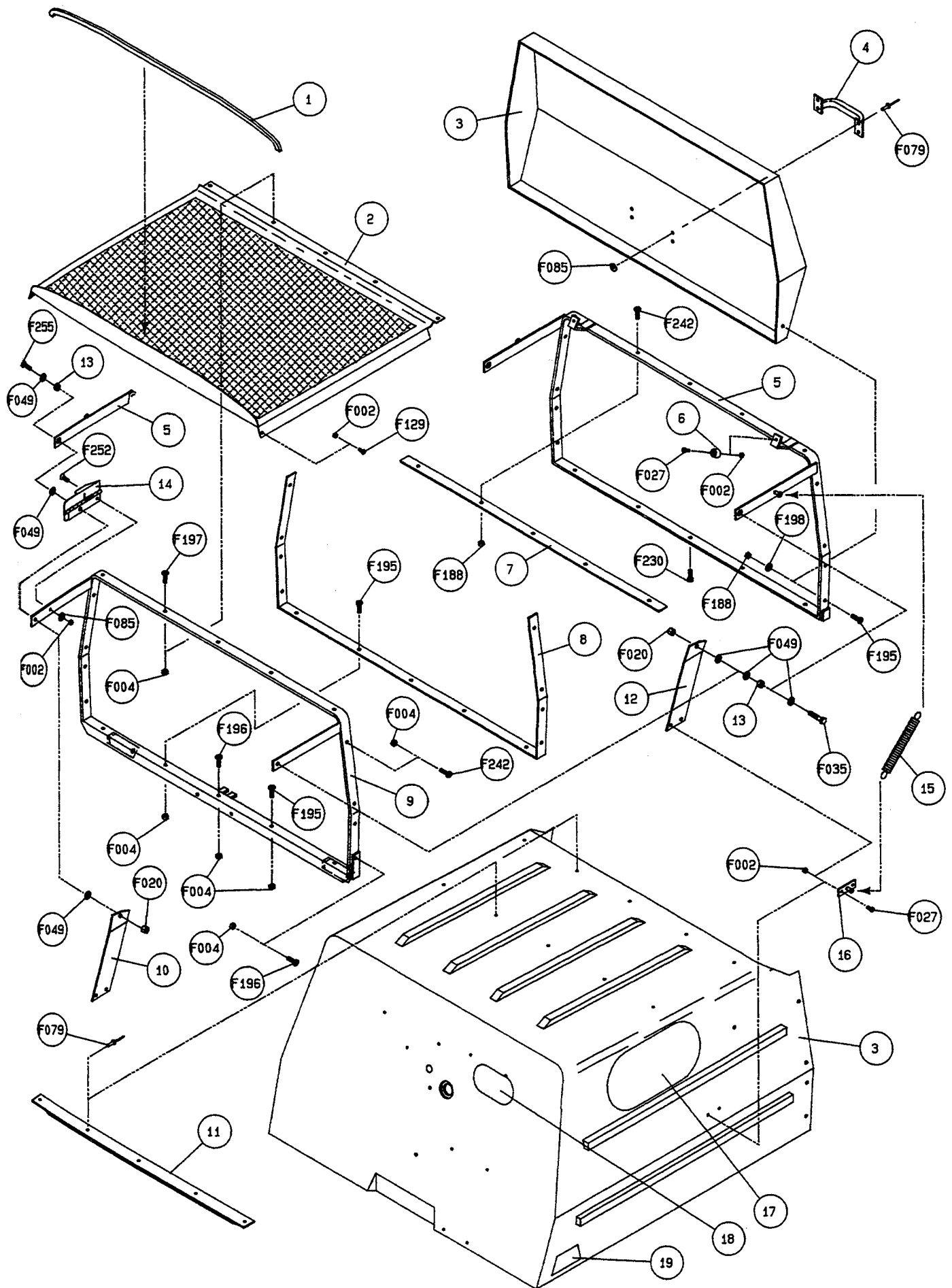
Figure G1 – GHS 7.0 Bushel Catcher Assembly
