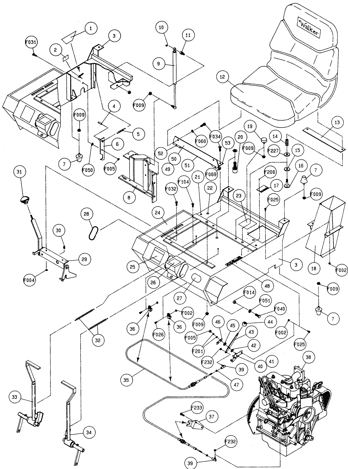
Figure B1 – Front Body Assembly
