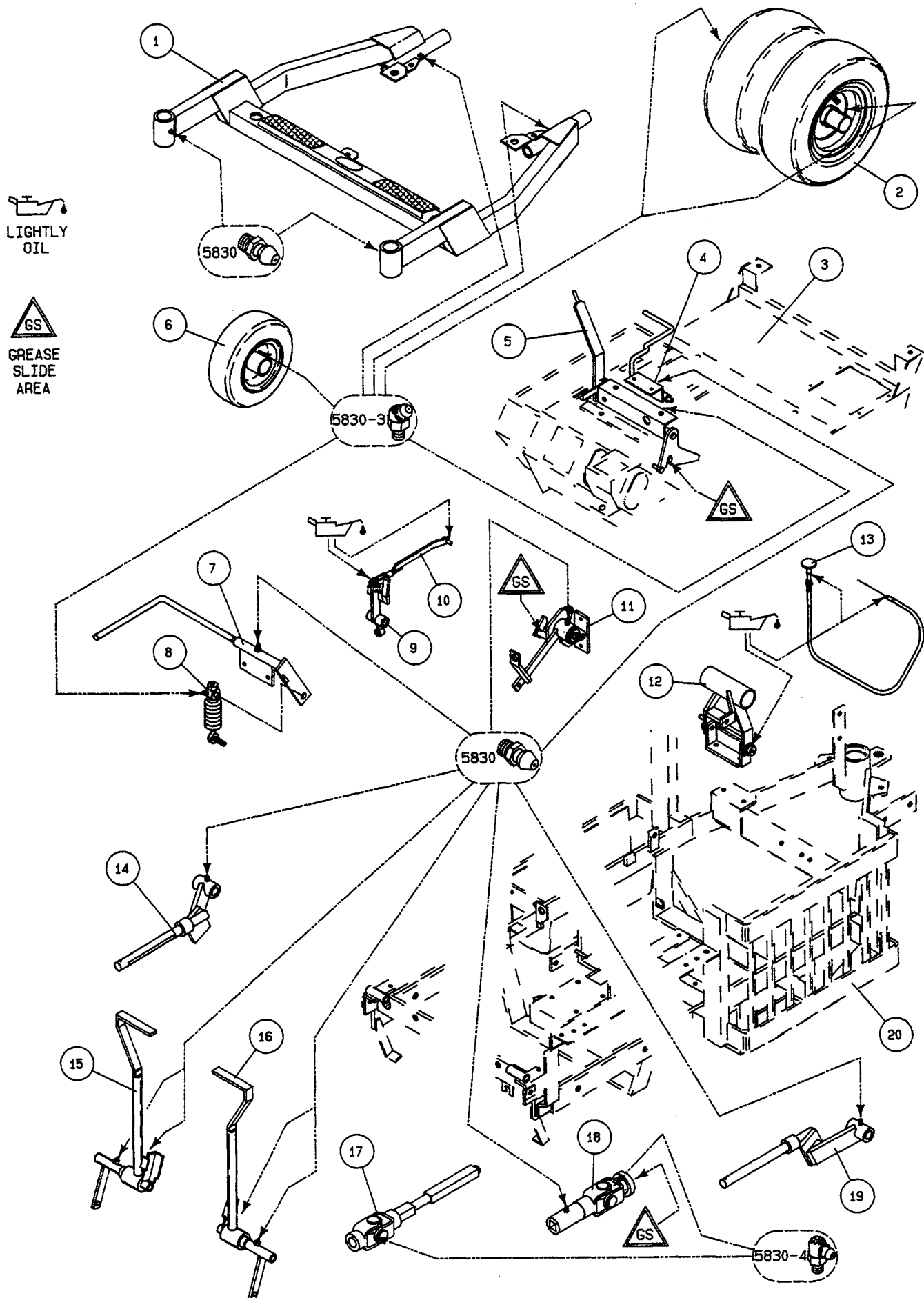
Figure L1 – Chassis Lubrication Points
