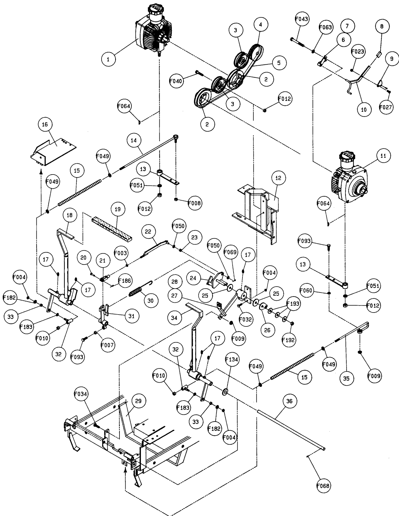
Figure C6 – Chassis Assembly (Steering Controls)
