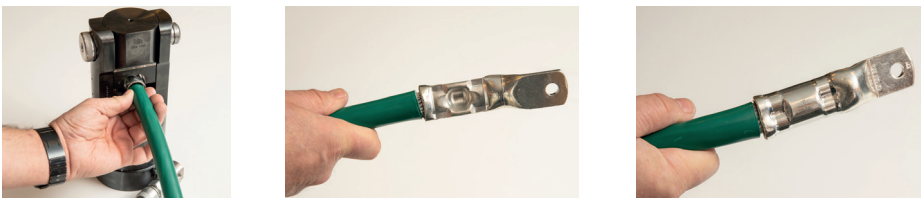
Crimping the DBI lug.
