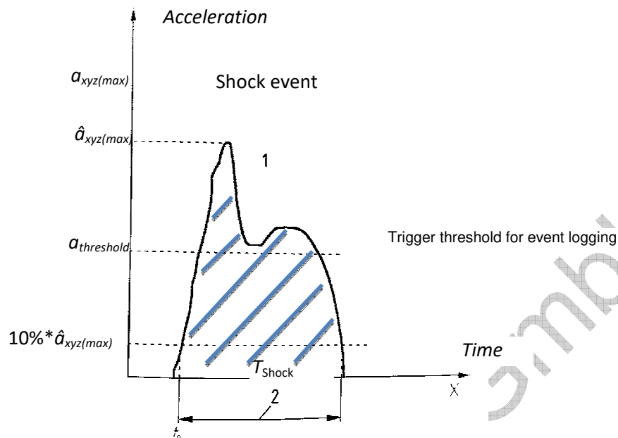
Figure 4: Typical sequence of a shock event
