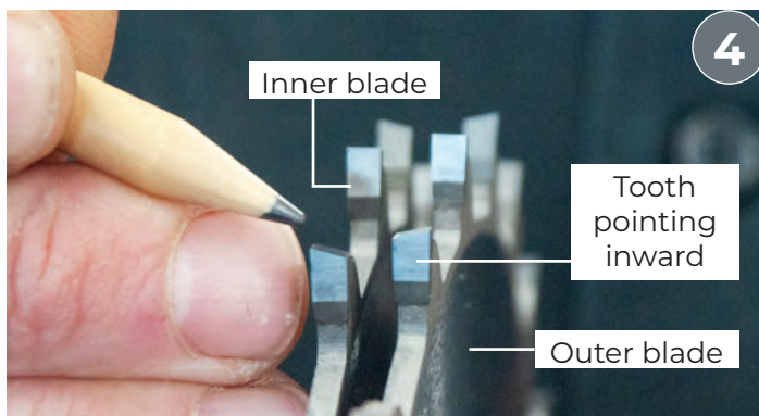
Make sure the teeth of the inner and outer blades are facing inward.
