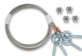
Ceiling Mounting Kit Code 400398
