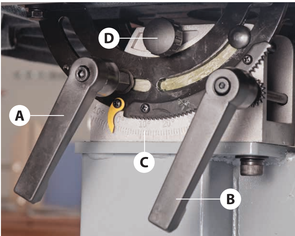
Tilt quadrant clamping handle (A), Table adjusting handle (B), Tilt quadrant scale (C), Lower thrust bearing adjusting knob (D)
