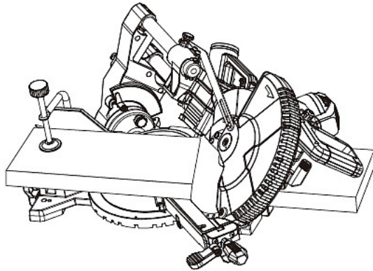
Fig. 41: Composite cut
