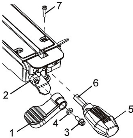
Fig. 7: Locking handle for the tilt angle
