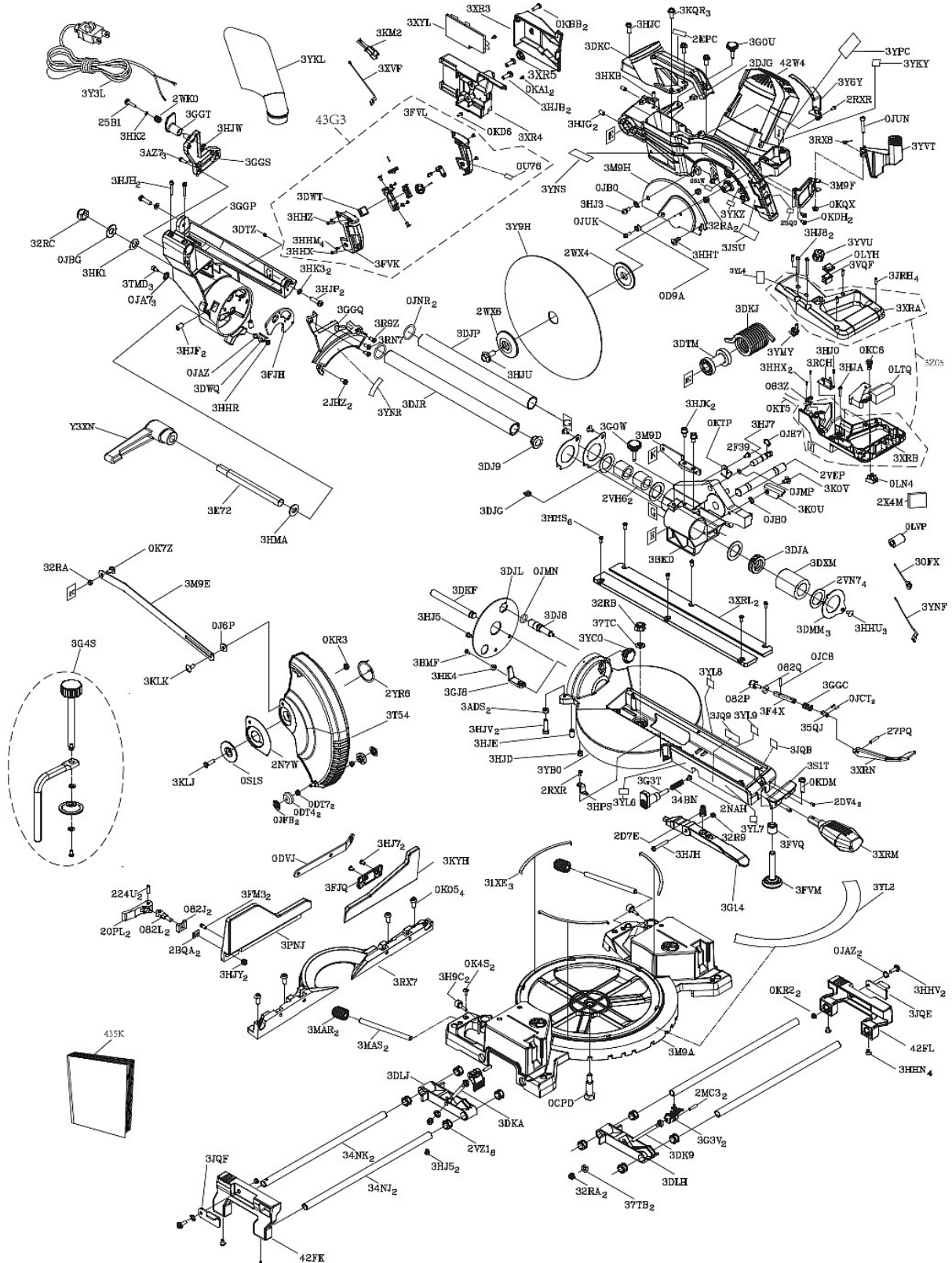
Fig. 50: Spare parts drawing 1 KGZ 2540 VARIO
