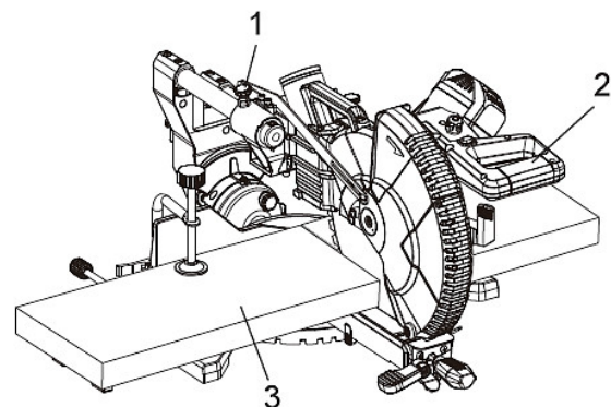
Fig. 45: Sliding cut
