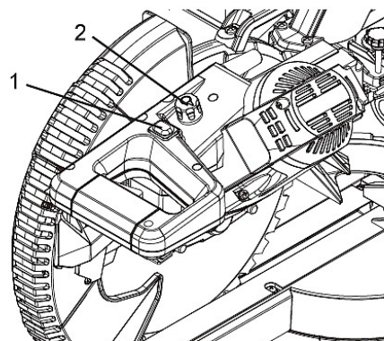
Fig. 29: Switch for varying the speed
