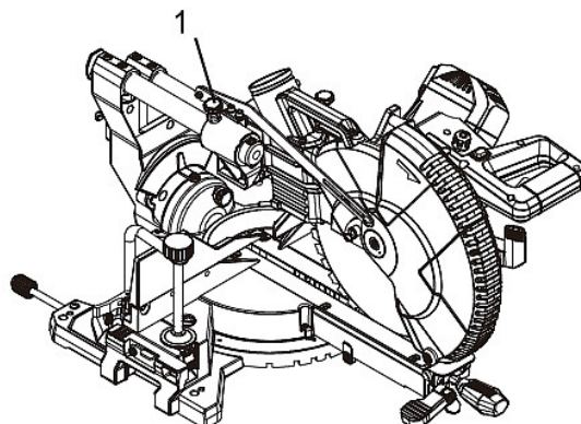
Fig. 11: Unlocking the sliding carriage
