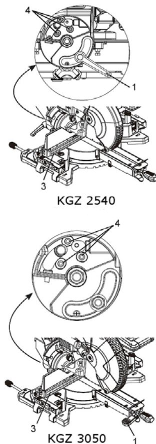
Fig. 18: Setting the 90° inclination
