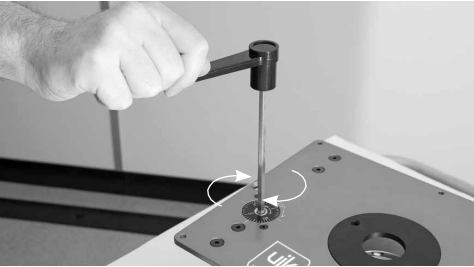
Turn the handle clock-wise to raise the table
