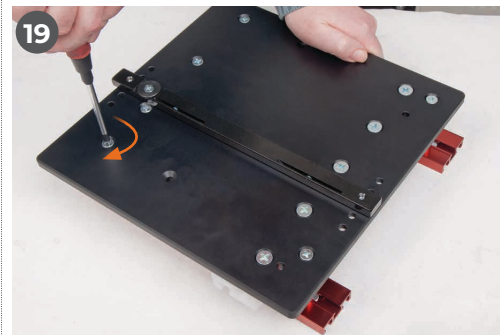
Turn the assembly over and tighten all the fixings
