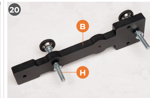
Remove the handles and the two nuts from assembly (H). Introduce the threads through the holes in assembly (B) as illustrated and replace the nuts
