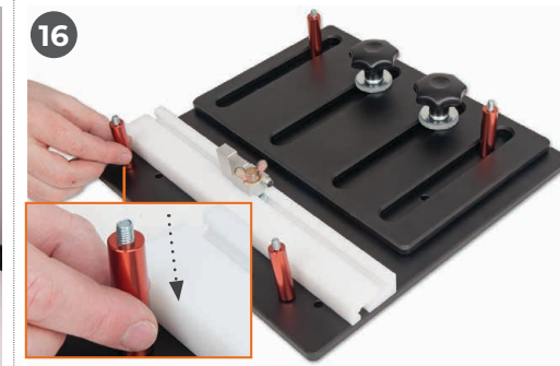
Introduce the height spacer tubes down over the four threads as shown
