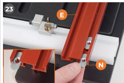
Insert two oval nuts (N) into the 'T' slot to the end of guide rail (E), see illustration above. Repeat for the remaining oval nut but to the opposite rail
