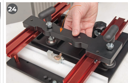
Lower the clamping beam assembly (B) as shown, down over the two rails (E) and line up the threaded holes in oval nuts (N) with the three pre-drilled holes in the beam assembly
