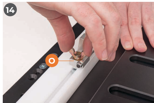
Manoeuvre the 'Adjustable Stop' (O) to the centre of assembly (F) and lightly tighten the butterfly nut
